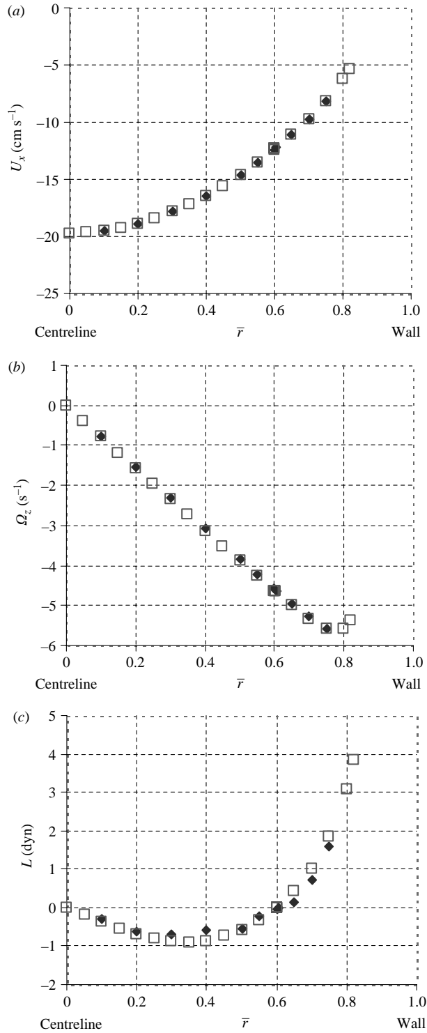
FIGURE 3. The steady-state values of the particle velocities (a) U_x and (b) \Omega_z and (c) the lift force L , from the constrained simulation at different radial positions. The □, ALE and ◆, DLM results are in good agreement.
